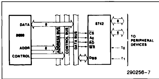
Figure 3. 8088-8742 interface
