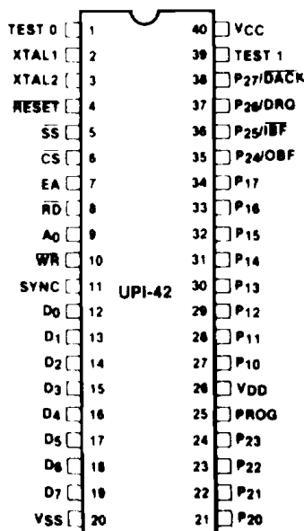
Figure 1. Pin Configuration
