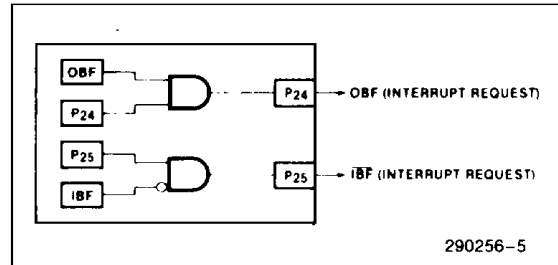
Data Bus Buffer Interrupt Capability
