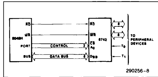
Figure 4. 8048H-8742 interface
