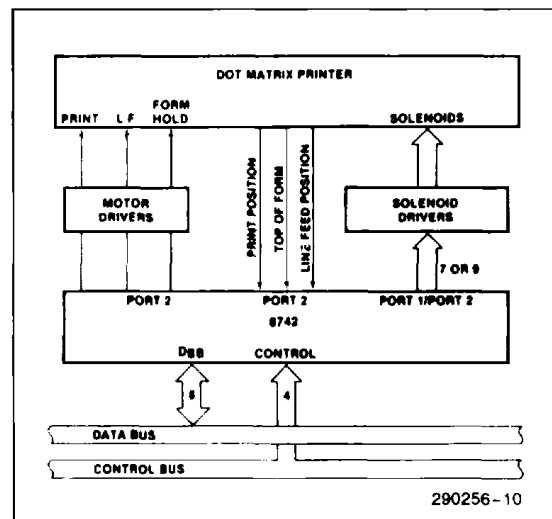
Figure 6. 8742 80-Column Matrix Printer interface
