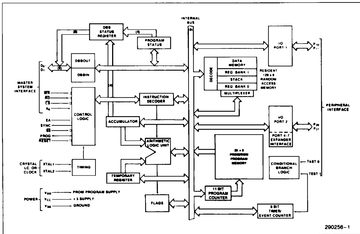
Figure 2. Block Diagram
