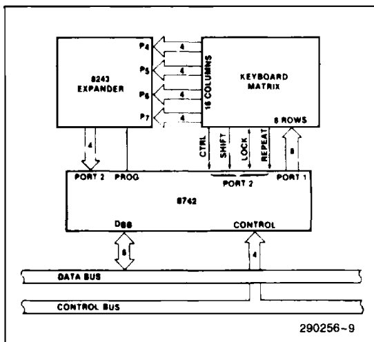
Figure 5. 8742-8243 Keyboard Scanner
