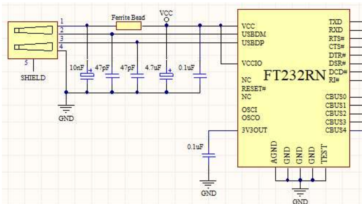
Figure 6.1 Illustrates the FT232RN in a typical USB bus powered design configuration. A USB bus powered device gets its power from the USB bus. Basic rules for USB bus power devices are as follows –
