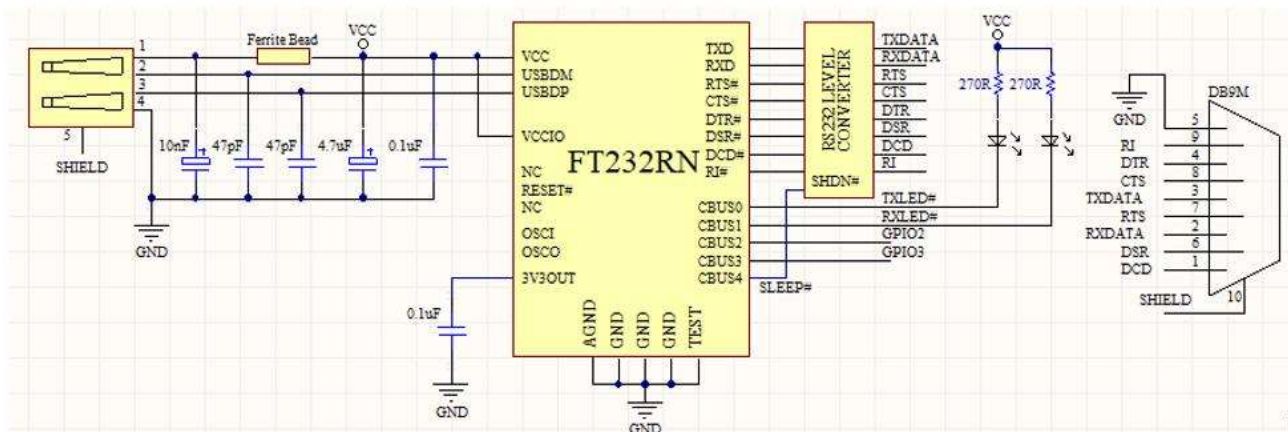
Figure 7.1 Application Example showing USB to RS232 Converter
