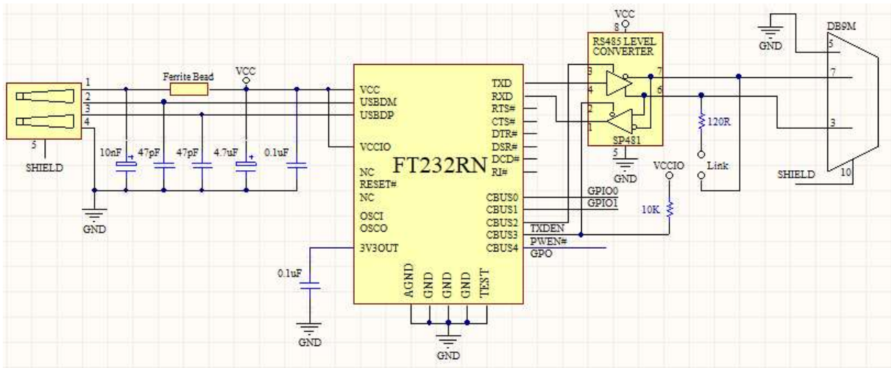
Figure 7.2 Application Example Showing USB to RS485 Converter
