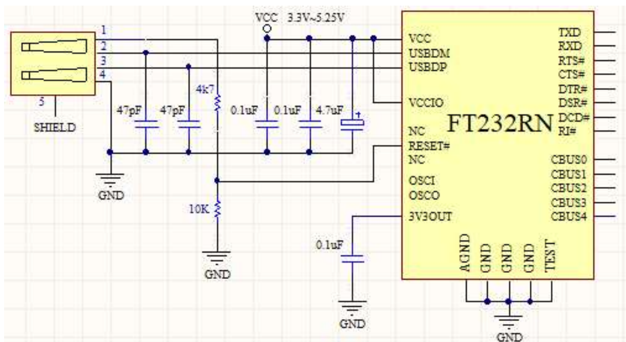
Figure 6.2 Self-Powered Configuration
